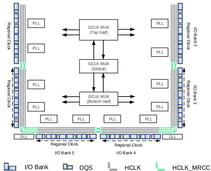
Figure 2-1 Clock Resources (138K / 75K)
