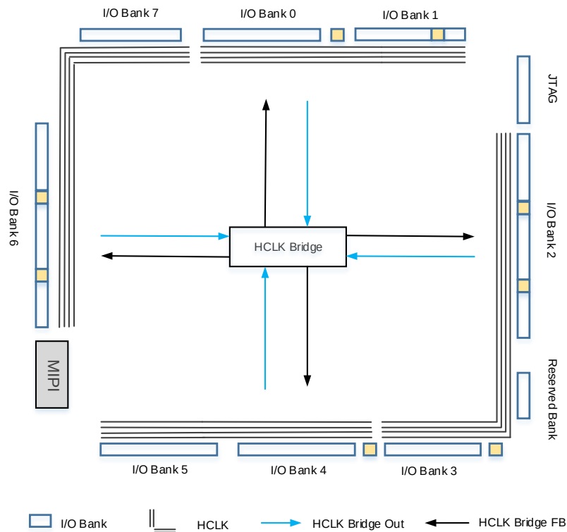
Figure 2-8 HCLK Structure View (15K)
