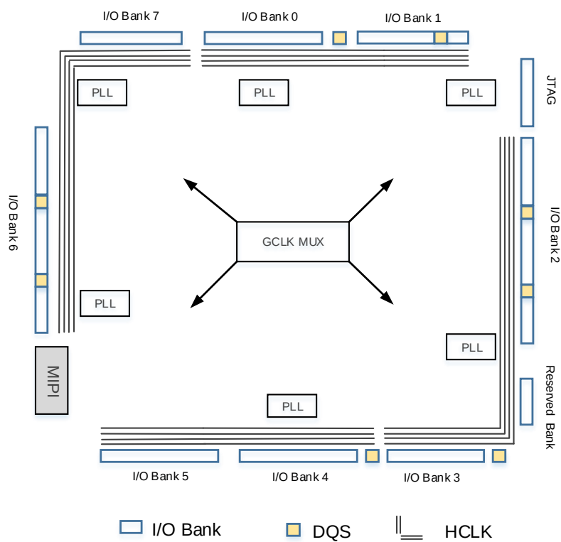
Figure 2-3 Clock Resources (25K)
