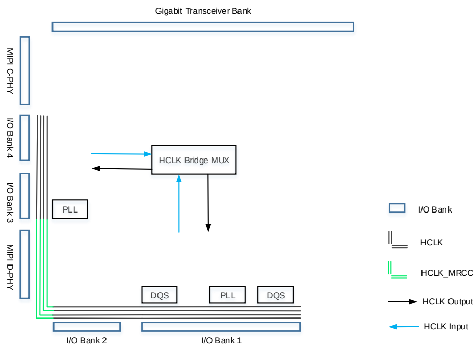
Figure 2-8 HCLK Structure View (15K)
