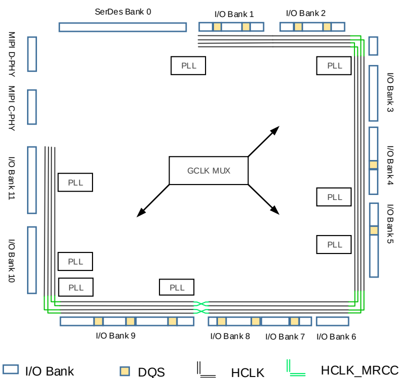
Figure 2-3 Clock Resources (25K)
