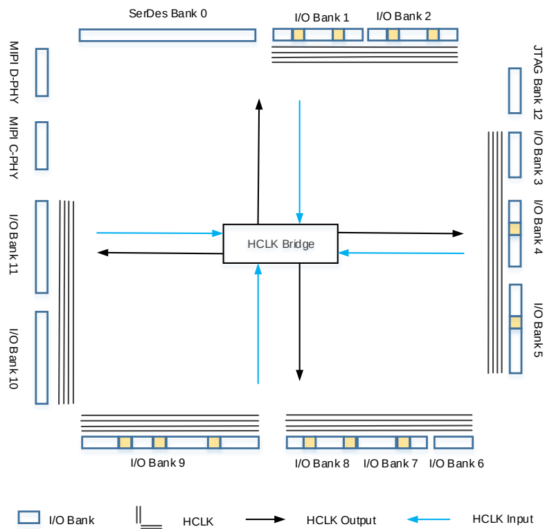
Figure 2-6 HCLK Structure View (60K)
