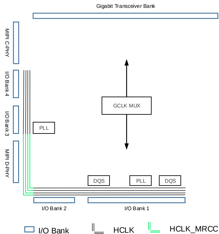
Figure 2-4 Clock Resources (15K)
