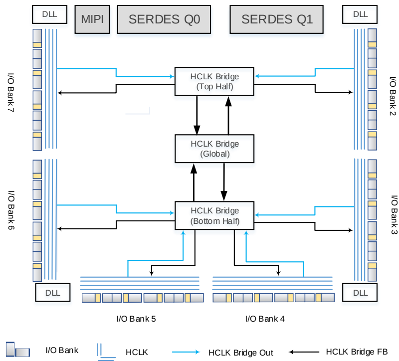
Figure 2-6 HCLK Structure View (60K)
