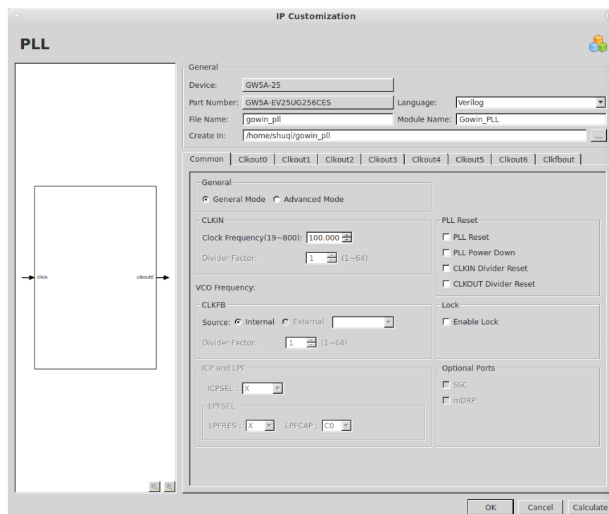
Figure 5-10 IP Customization of PLLA
